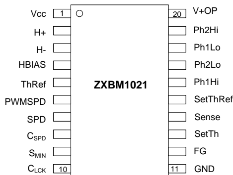
QSOP-20
