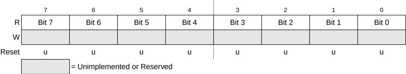
Figure 19-7. Debug Trace Buffer Register Low (DBGTBBL)
