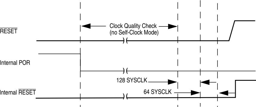
Figure 5-27. \overline{\text{RESET}} Pin Held Low Externally
