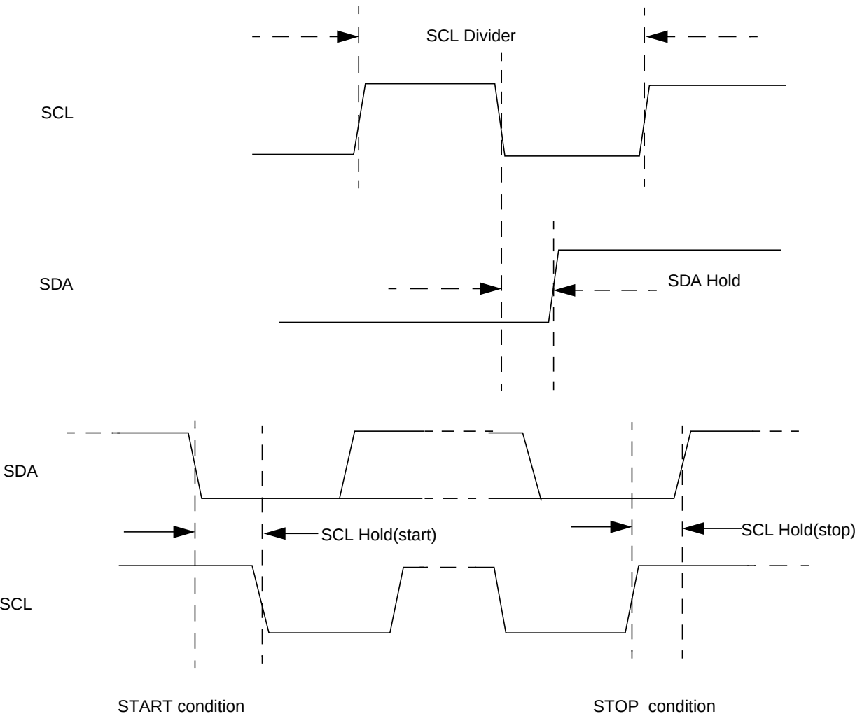
Figure 11-4. SCL Divider and SDA Hold
