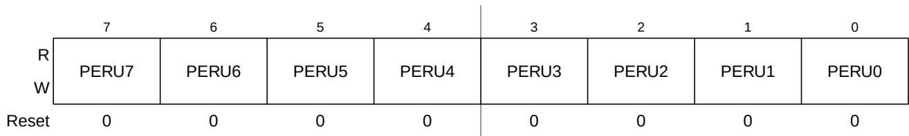
Figure 4-47. Port U Pull Device Enable Register (PERU)
