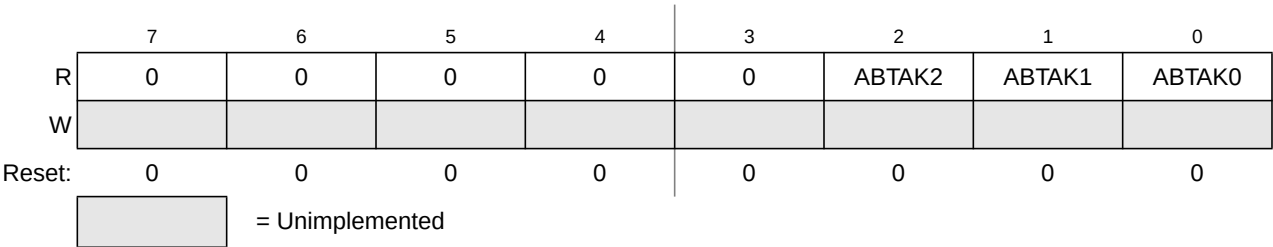
Figure 12-11. MSCAN Transmitter Message Abort Acknowledge Register (CANTAAB)
