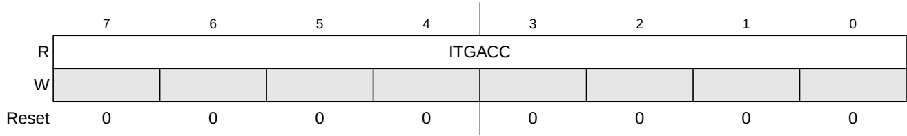
Figure 10-9. Integration Accumulator Register Low (ITGACC)
