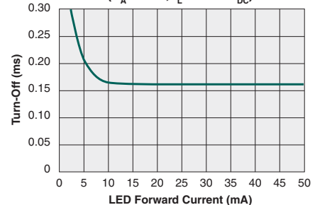
Typical Turn-Off vs. LED Forward Current ( T_A=25^\circ\text{C} , I_L=120\text{mA}_{\text{DC}} )
