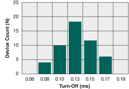
Typical Turn-Off Time (N=50, T A =25°C, I L =120mA DC , I F =5mA)
