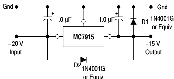
Figure 11. Protection Diodes
