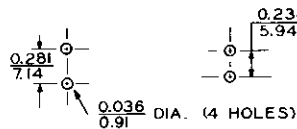
SUGGESTED MOUNTING HOLES
