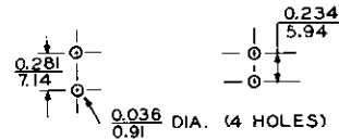
SUGGESTED MOUNTING HOLES
