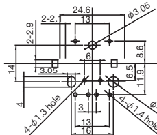
Recommended Hole Dimension (t = 1.6)
