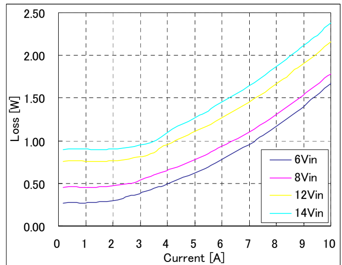
Fig-3.3V-3: Power Loss vs. load current and input voltage for Vout=3.3V. Airflow rate=200 LFM (1m/s) and Ta=25°C.
