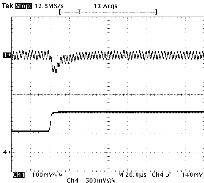
Fig-5.0V-6: Output voltage response for V_{out}=5.0V to positive load current step change from 5A to 10A with slew rate of 5A/us at V_{in}=12V . C_o=47\mu F \times 2 ceramic. Top trace: output voltage (100mV/div.) Bottom trace: load current (5A/div.) Time scale: 20us/div.
