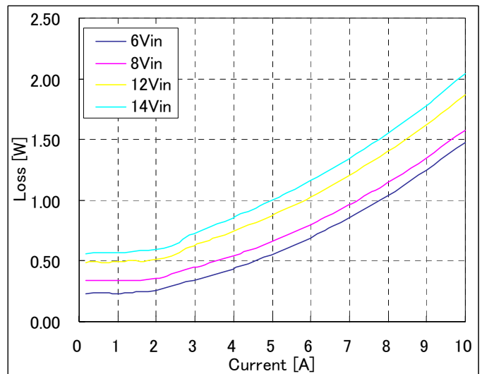
Fig-2.0V-3: Power Loss vs. load current and input voltage for Vout=2.0V. Airflow rate=200 LFM (1m/s) and Ta=25°C.
