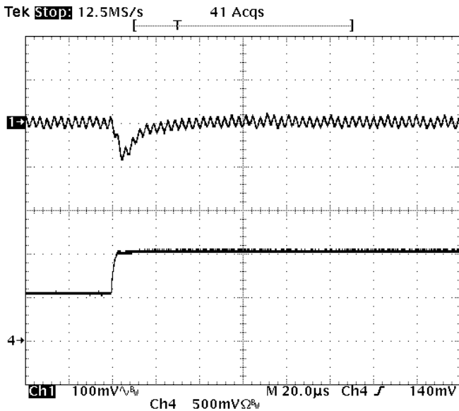
Fig-2.5V-6: Output voltage response for V_{out}=2.5V to positive load current step change from 5A to 10A with slew rate of 5A/us at V_{in}=12V . C_o=47\mu F \times 2 ceramic. Top trace: output voltage (100mV/div.) Bottom trace: load current (5A/div.) Time scale: 20us/div.
