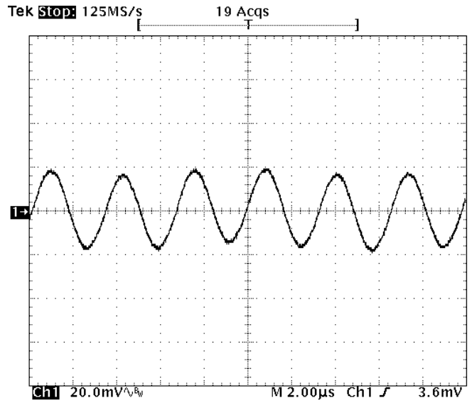
Fig-5.0V-5: Output voltage ripple (20mV/div.) for V_{out}=5.0V at full rated load current into a resistive load with external capacitance 47\mu F \times 2 ceramic + 1\mu F ceramic at V_{in}=12V . Time scale: 2 us/div
