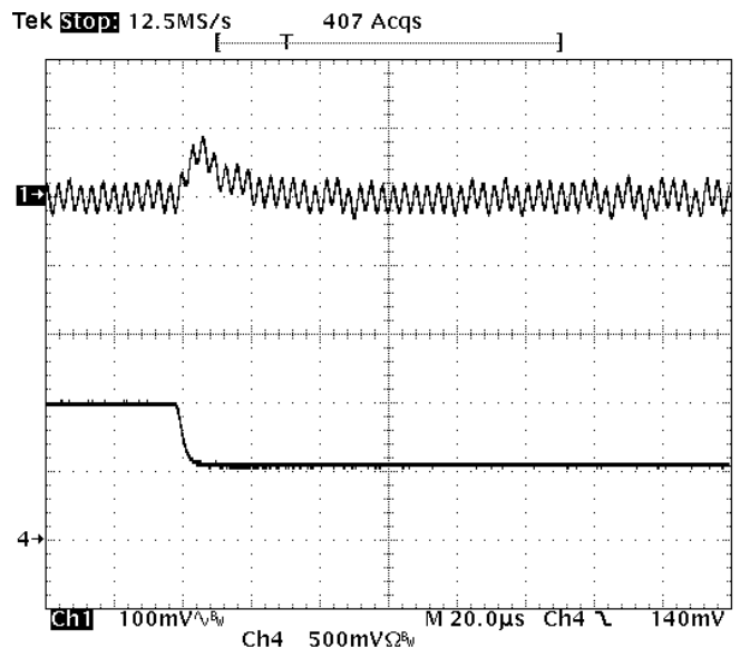
Fig-5.0V-7: Output voltage response for V_{out}=5.0V to negative load current step change from 10A to 5A with slew rate of -5A/us at V_{in}=12V . C_o=47\mu F \times 2 ceramic. Top trace: output voltage (100mV/div.) Bottom trace: load current (5A/div.) Time scale: 20us/div.
