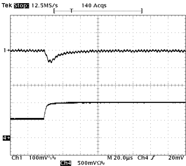
Fig-1.0V-6: Output voltage response for V_{out}=1.0V to positive load current step change from 5A to 10A with slew rate of 5A/us at V_{in}=12V . C_o=47\mu F \times 2 ceramic. Top trace: output voltage (100mV/div.) Bottom trace: load current (5A/div.) Time scale: 20us/div.
