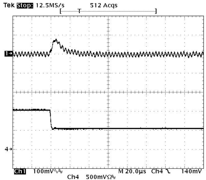
Fig-2.5V-7: Output voltage response for V_{out}=2.5V to negative load current step change from 10A to 5A with slew rate of -5A/us at V_{in}=12V . C_o=47\mu F \times 2 ceramic. Top trace: output voltage (100mV/div.) Bottom trace: load current (5A/div.) Time scale: 20us/div.
