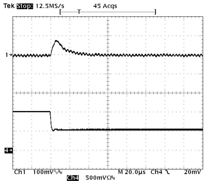
Fig-1.0V-7: Output voltage response for V_{out}=1.0V to negative load current step change from 10A to 5A with slew rate of -5A/us at V_{in}=12V . C_o=47\mu F \times 2 ceramic. Top trace: output voltage (100mV/div.) Bottom trace: load current (5A/div.) Time scale: 20us/div.
