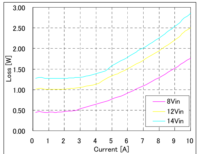
Fig-5.0V-3: Power Loss vs. load current and input voltage for Vout=5.0V. Airflow rate=200 LFM (1.0 m/s) and Ta=25°C.
