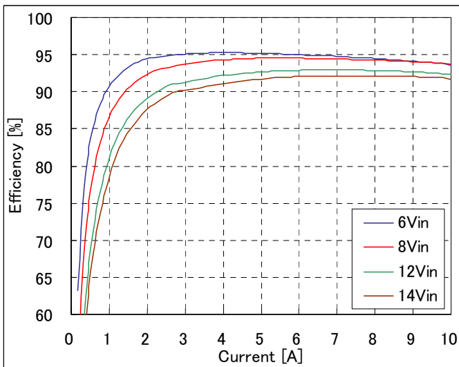
Fig-2.5V-2: Efficiency vs. load current and input voltage for V_{out}=2.5V . Airflow rate=200 LFM (1m/s) and T_a=25^{\circ}C .
