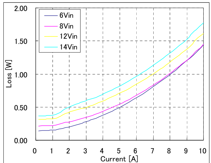
Fig-1.0V-3: Power Loss vs. load current and input voltage for Vout=1.0V. Airflow rate=200 LFM (1m/s) and Ta=25°C.
