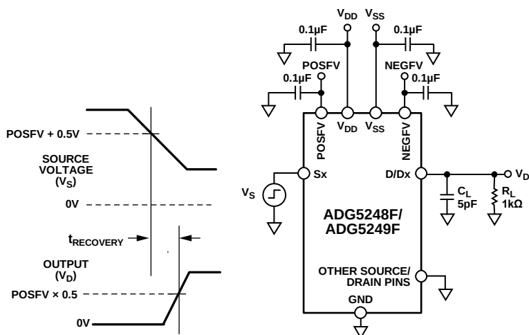
Figure 44. Overvoltage Recovery Time, t_{RECOVERY}
