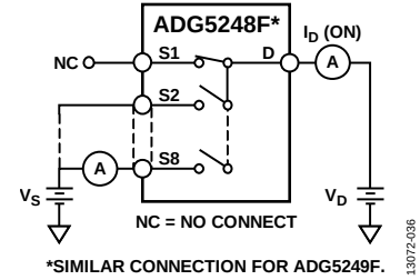
Figure 37. On Leakage
