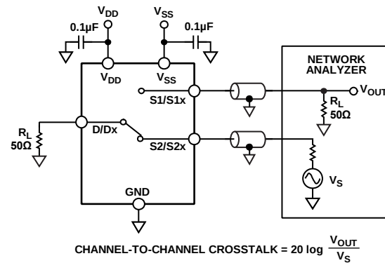
Figure 40. Channel-to-Channel Crosstalk
