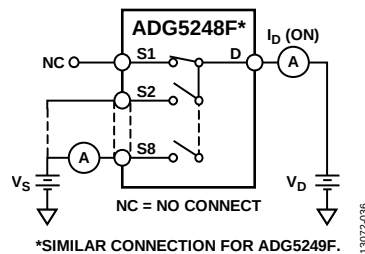
Figure 37. On Leakage
