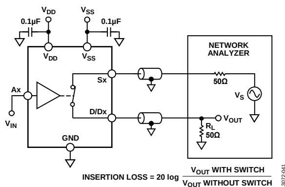
Figure 42. Bandwidth
