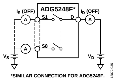
Figure 36. Off Leakage
