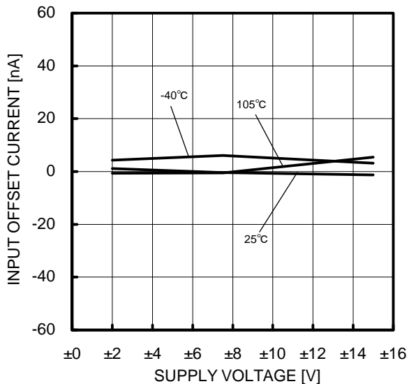
Fig.36 Input Offset Current - Supply Voltage (Vicm=0V, Vout=0V)
