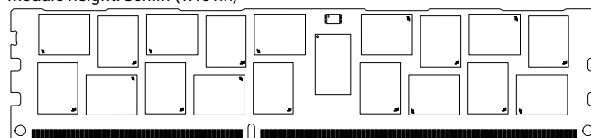
Figure 1: 240-Pin RDIMM (MO-269 R/C E2)
