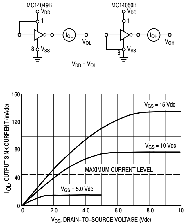
Figure 2. Typical Output Sink Characteristics
