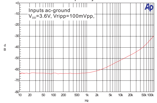
10. PSRR VS Frequency
