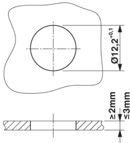
Panel cutout
