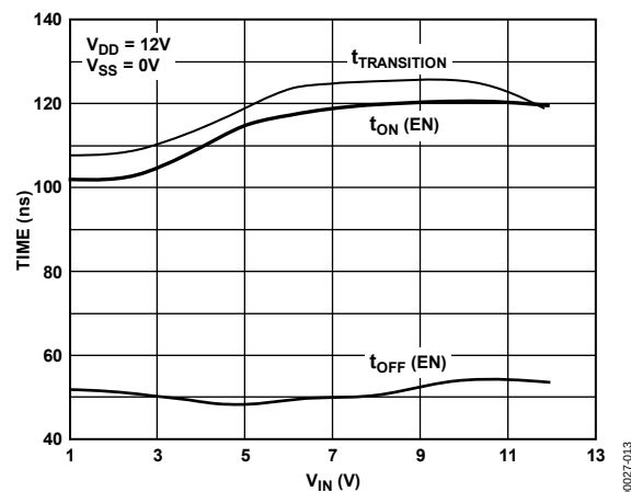
Figure 13. Switching Time vs. V_{\text{IN}} (Single Supply)
