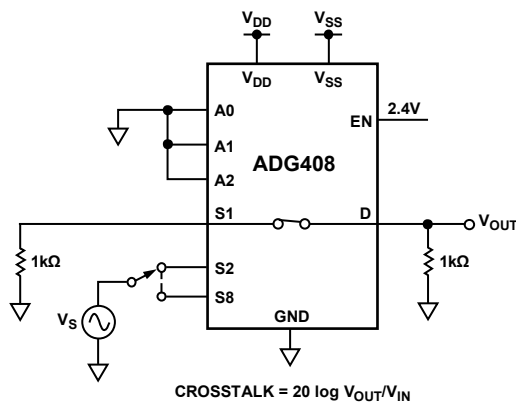
Figure 27. Channel-to-Channel Crosstalk
