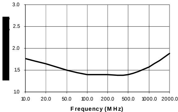
Insertion Loss
