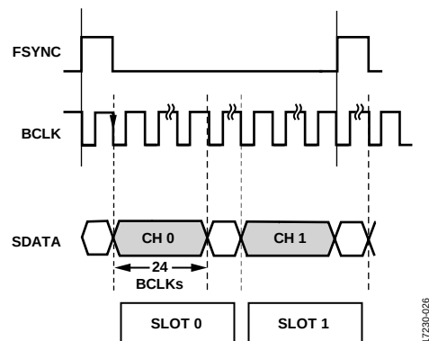
Figure 25. TDM-2, I²C Mode, One BCLK Delay, Normal Clock Polarity, Default Channel Assignments
