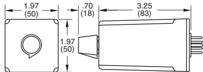
Outline Dimensions
