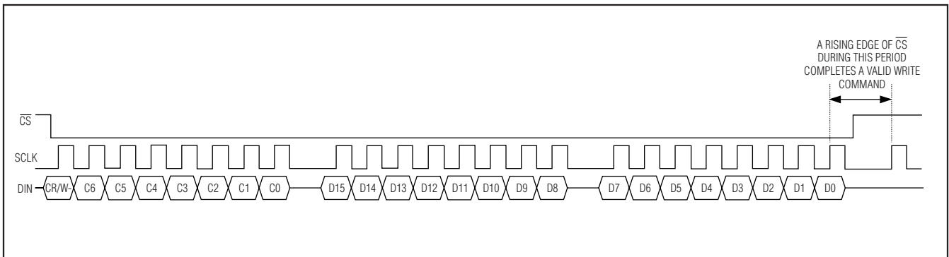
Figure 2. SPI Write Sequence
