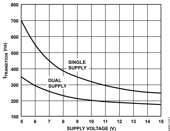
Figure 10. t_{\text{TRANSITION}} vs. Supply Voltage: Dual and Single Supplies, T_A = 25^\circ\text{C} (Note: For V_{DD} and V_{SS1} < 10\text{V} ; V_1 = V_{DD}/V_{SS} , V_2 = V_{SS}/V_{DD} . (see Figure 19))
