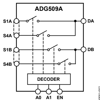
Figure 2. ADG509A
