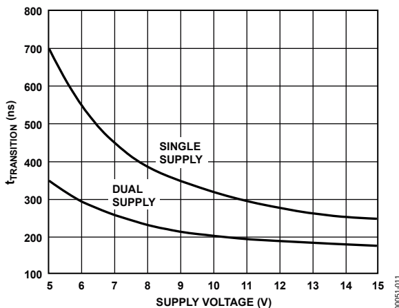
Figure 10. t_{\text{TRANSITION}} vs. Supply Voltage: Dual and Single Supplies, T_A = 25^\circ\text{C} (Note: For V_{DD} and V_{SS} < 10 V; V_1 = V_{DD}/V_{SS} , V_2 = V_{SS}/V_{DD} . (see Figure 19))
