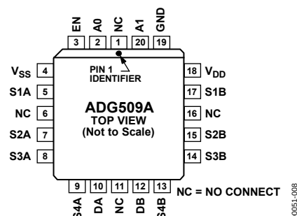
Figure 7. ADG509A PLCC
