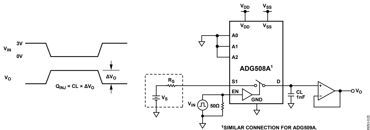
Figure 22. Charge Injection
