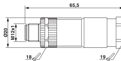
Dimensioned drawing
