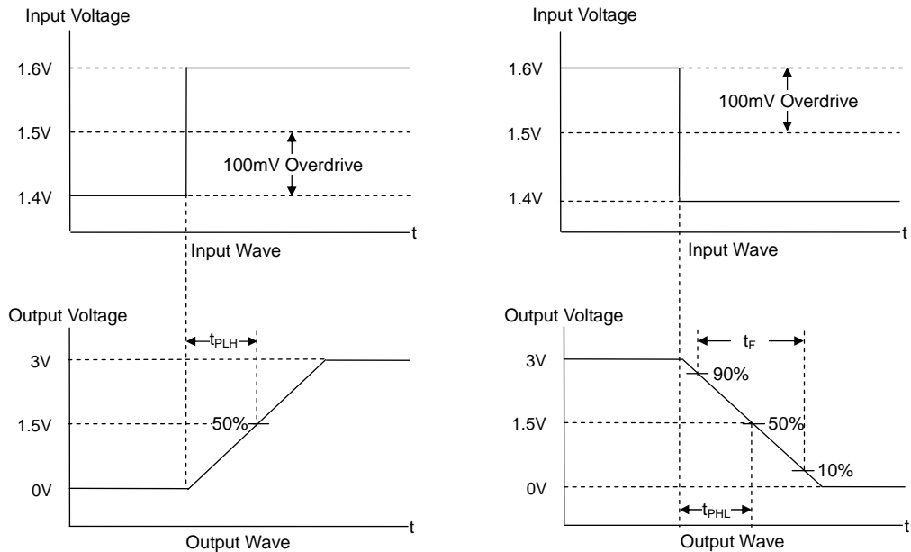
Figure 43. Response Time Input and Output Wave
