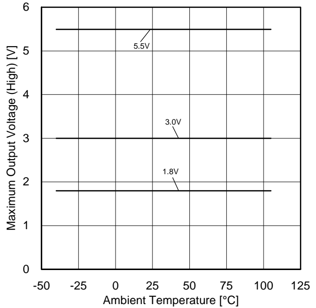
Figure 26. Maximum Output Voltage (High) vs Ambient Temperature ( R_L=10k\Omega , V_{RL}=V_{DD} )
