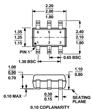
Figure 20. 6-Lead Thin Shrink Small Outline Transistor Package [SC70]
