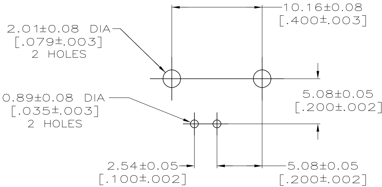
PCB CONFIGURATION
