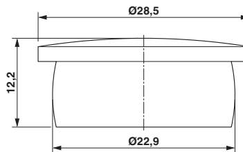
Dimensioned drawing
