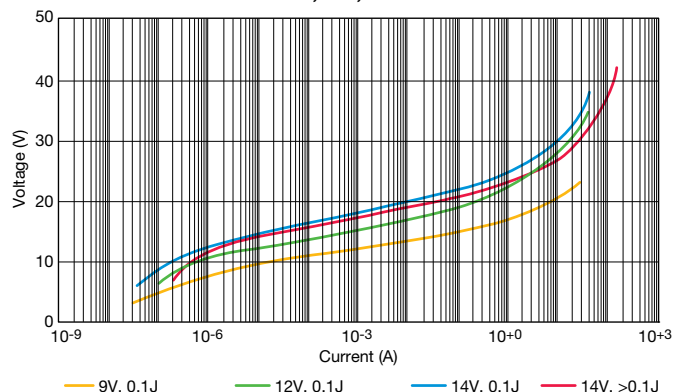
VI Curves - 9V, 12V, and 14V Products
