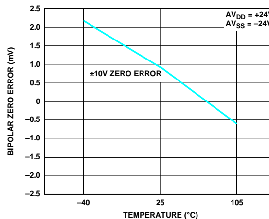
Figure 10. Bipolar Zero Error vs. Temperature
