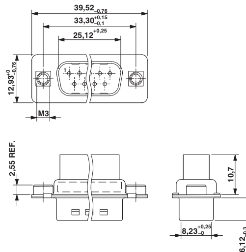
Dimensioned drawing
