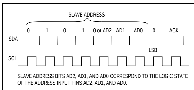
Figure 5. Address Byte
