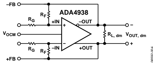
Figure 57. Circuit Definitions
