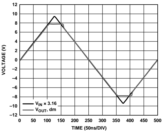
Figure 39. Overdrive Amplitude Characteristics (Triangle Wave Input)
