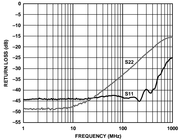
Figure 35. Return Loss (S11, S22) vs. Frequency
