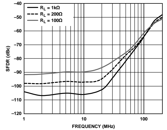
Figure 36. SFDR vs. Frequency for Various Loads
