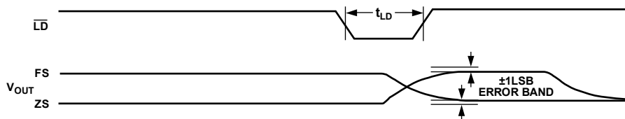
Figure 4. Output Transition
