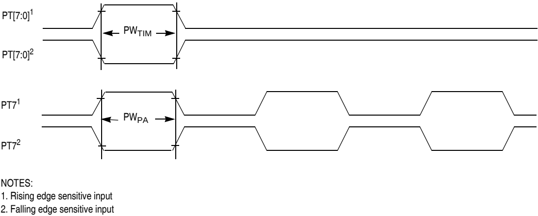
Figure 20-1. Timer Inputs
