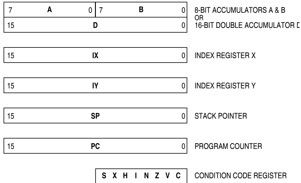
Figure 2-1. Programming Model
