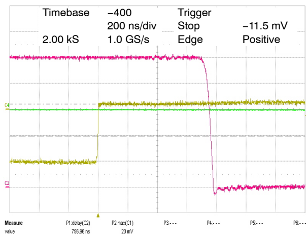
Figure 16. 10 mV Overdrive
