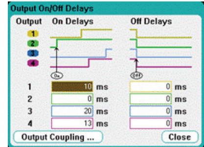
Figure 10. The Output On/Off Delays screen allows you to enter the delay times for each output. A graphical representation of the settings is shown to visually confirm your choices.
