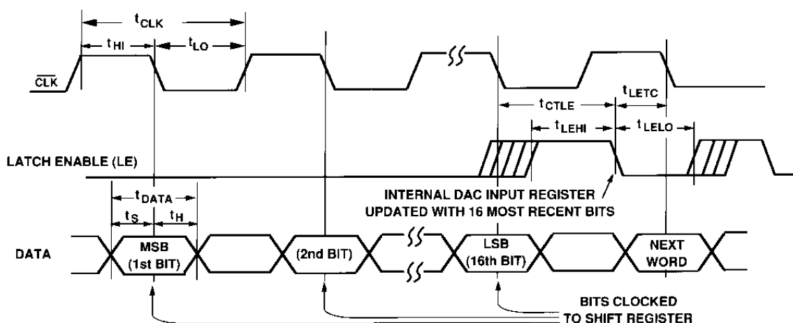
Figure 2. AD766 Serial Input Timing
