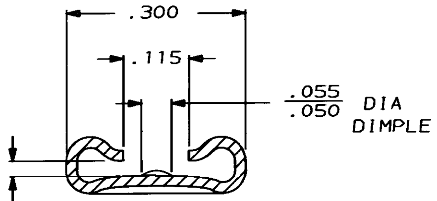
FITS .250 SERIES FASTON TAB SECTION A-A
