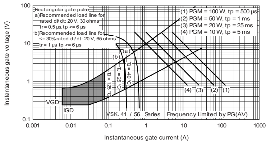
Fig. 22 - Gate Characteristics
