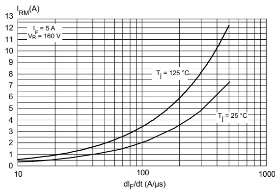
Figure 9. Peak reverse recovery current versus dl_F/dt (typical values, per diode)
