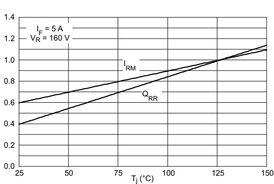
Figure 10. Dynamic parameters versus junction temperature (reference: T_i = 125^\circ\text{C} )
