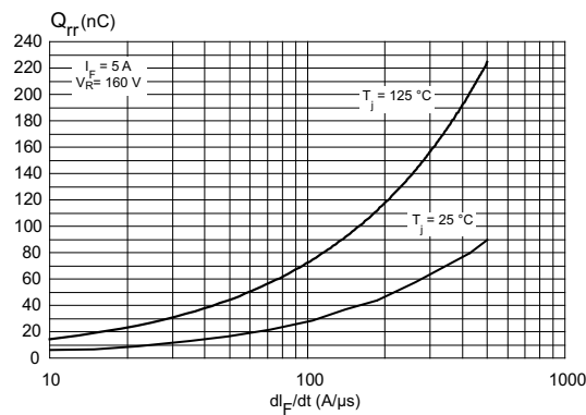
Figure 7. Reverse recovery charges versus dl_F/dt (typical values, per diode)
