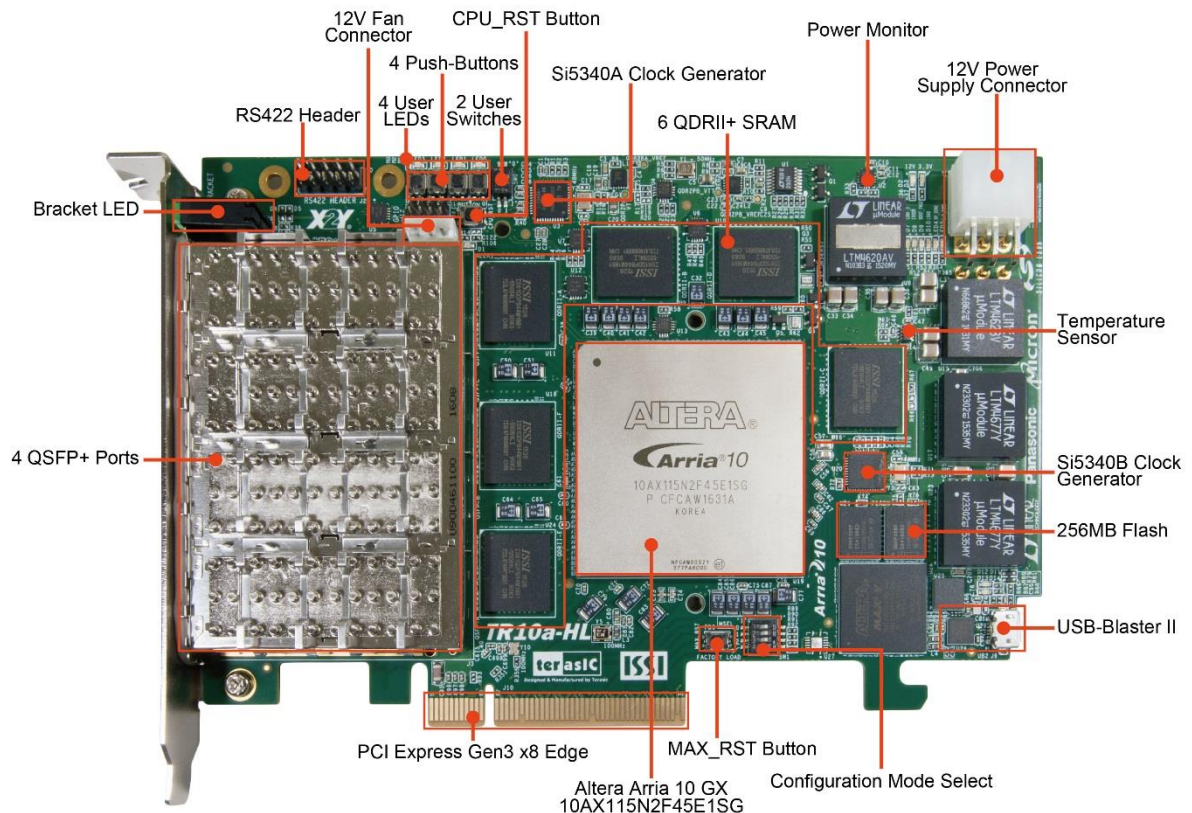
Figure 2-1 FPGA Board (Top)
