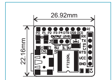
Figure 4: Dimensions of the board
